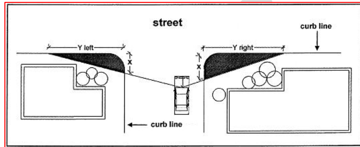
FIGURE 15-2018: INTERSECTION VISIBILITY
